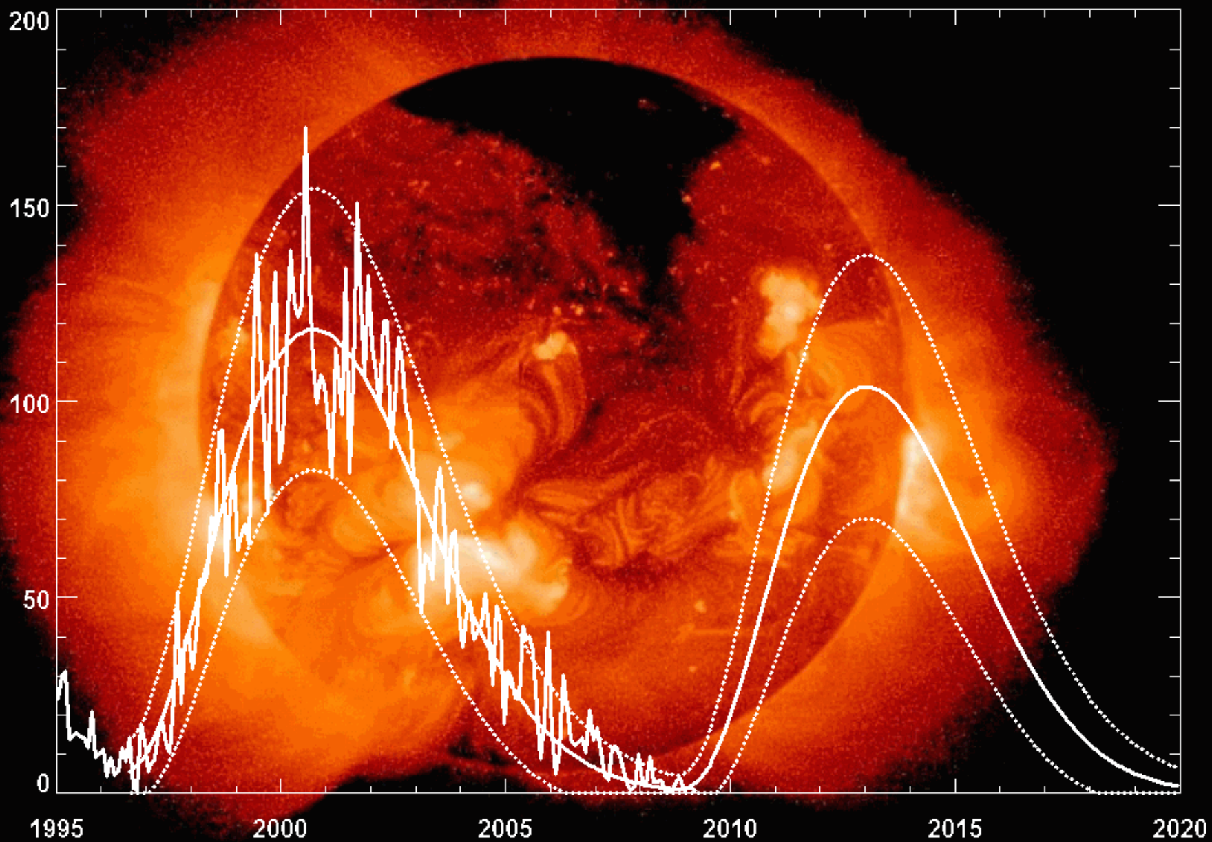
Cycle 23-24 Sunspot Number Prediction (April 2009)
