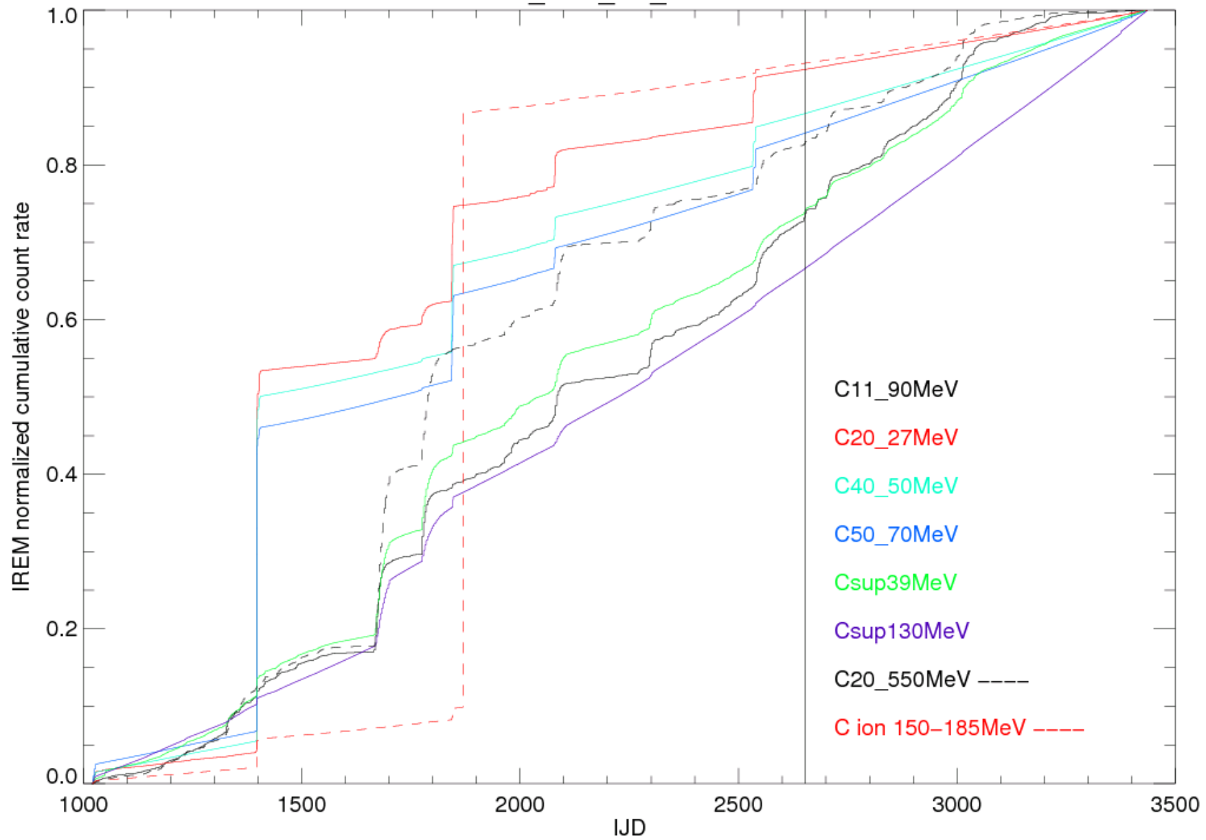
ibis_irem_cal_0009.fits
