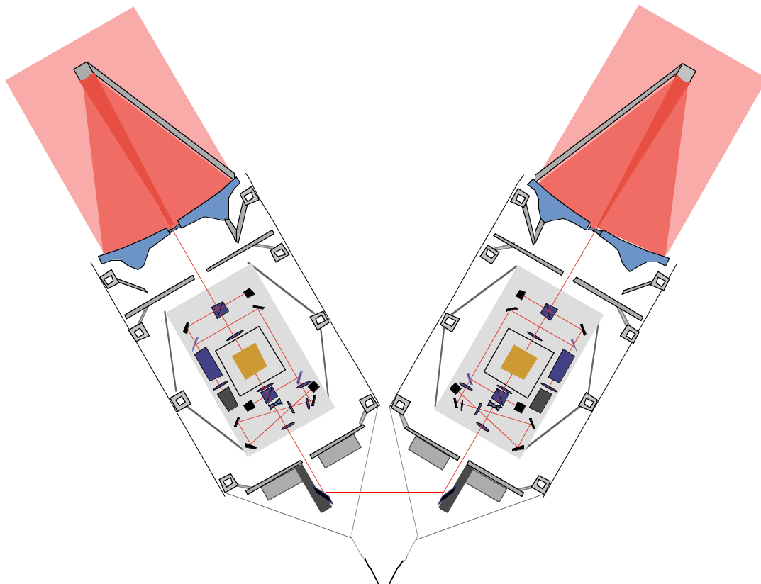
Figure 6-1 Cross section of the two optical assemblies comprising the main part of the payload on each LISA spacecraft. The two assemblies are mounted from flexures at the back (bottom of figure) and from pointing actuators (not shown) at the front, near the primary mirrors.
