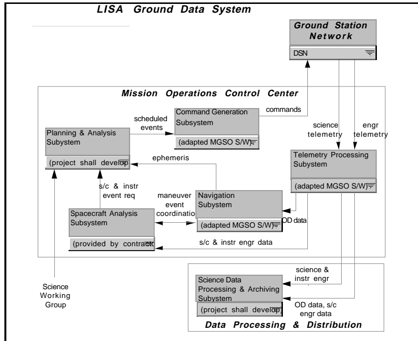
Figure 14-1 LISA ground data system.
